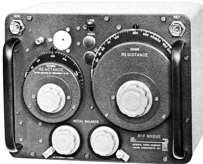
Figure 1a. Type 1606-A R-F Bridge.
