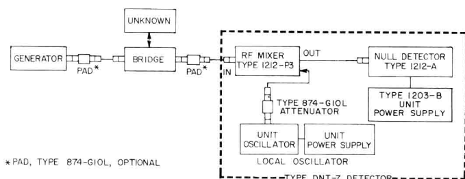
Figure 4. Block diagram of a typical system using the Type 1606-A R-F Bridge for impedance measurements between 3 and 50 Mc.
