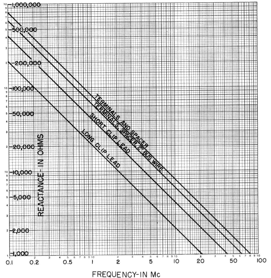
Figure 7. Capacitive Reactance to Ground of Connecting Leads as a Function of Frequency.
